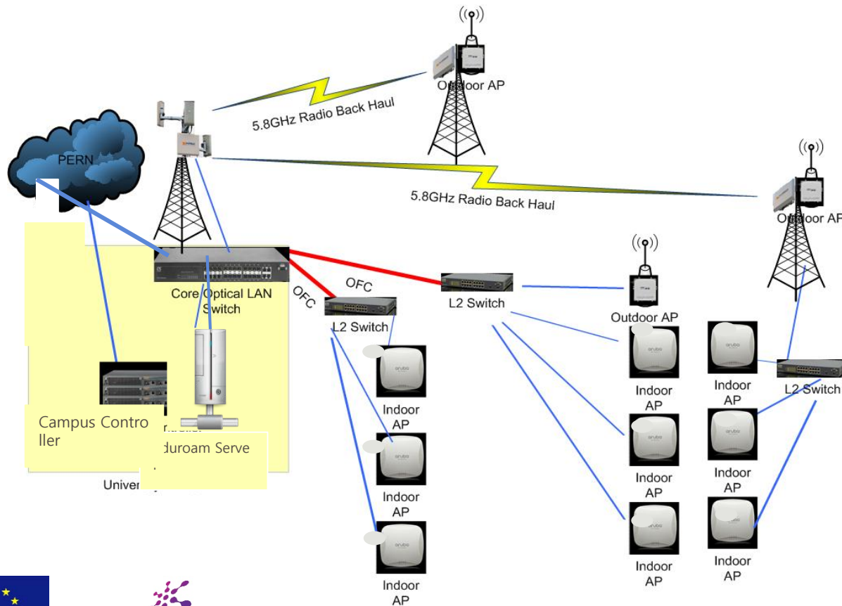
UNIVERSITY WIDE WiFi NETWORK DIAGRAM
